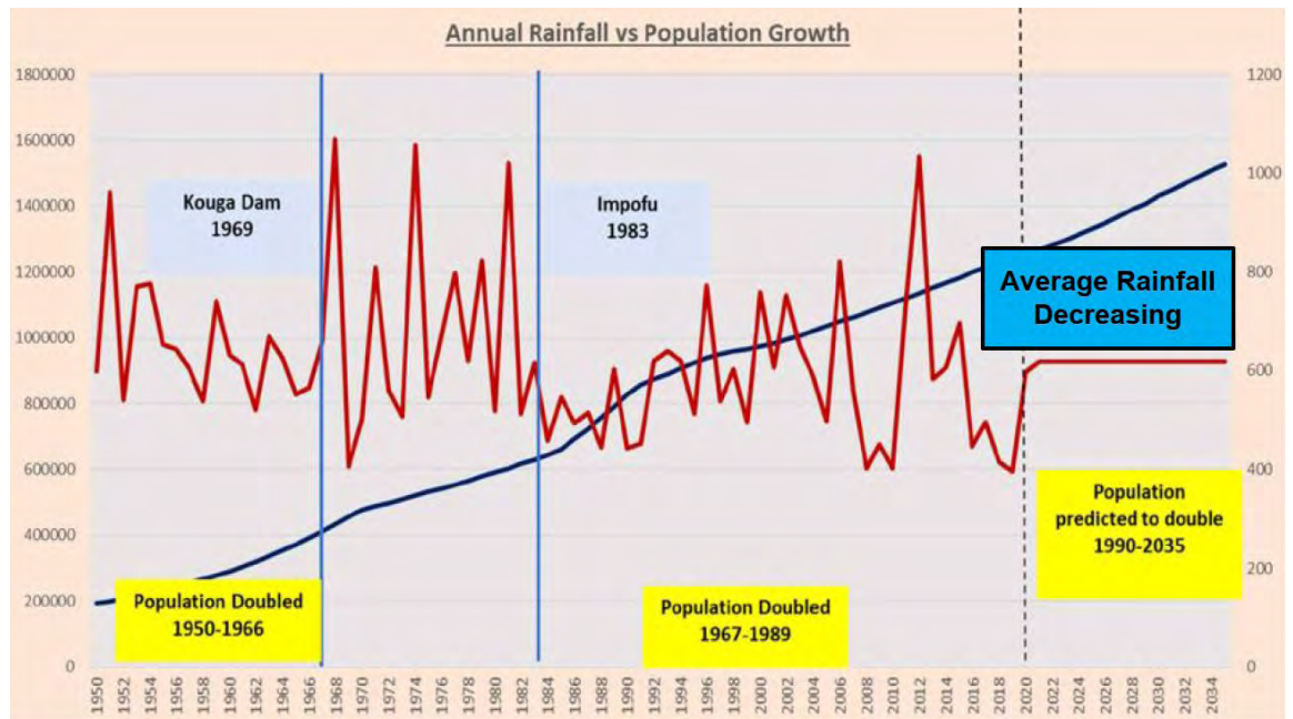
Figure 3-6. Historical water demand as compared to rainfall in the local catchments (NMBM, 2022b)
