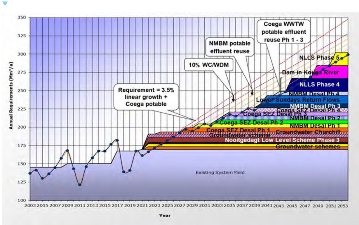
Figure 3-7. Comparison of future demands and supply options for NMBM potable water (Zutari, 2022)
