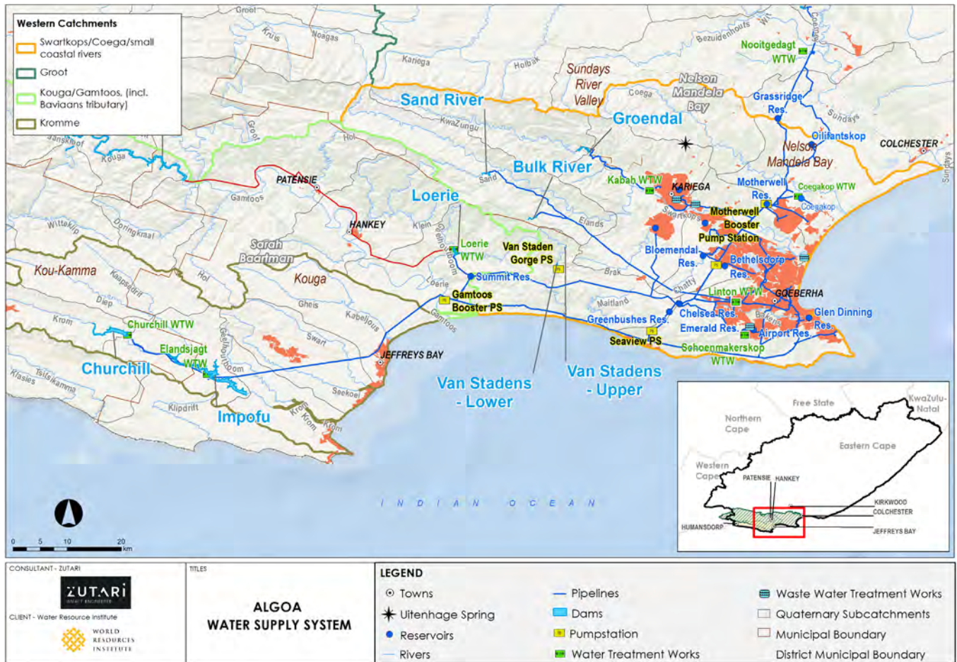
Figure 3-8. Water supply distribution network of NMBM
