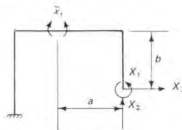
Fig. 7 A stress couple due to applied forces
