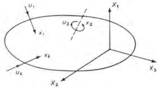
Fig. 2 Rigid body components of applied forces and displacements
