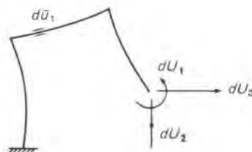
Fig. 10 Some typical distortions of a short length
