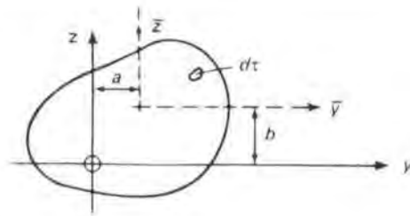
Fig. 13 Unsymmetrical cross-section
