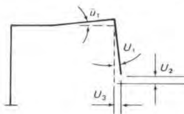
Fig. 8 Displacements due to corresponding rotation
