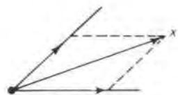
Fig. 3 Resolutes of a force in plane oblique axes
