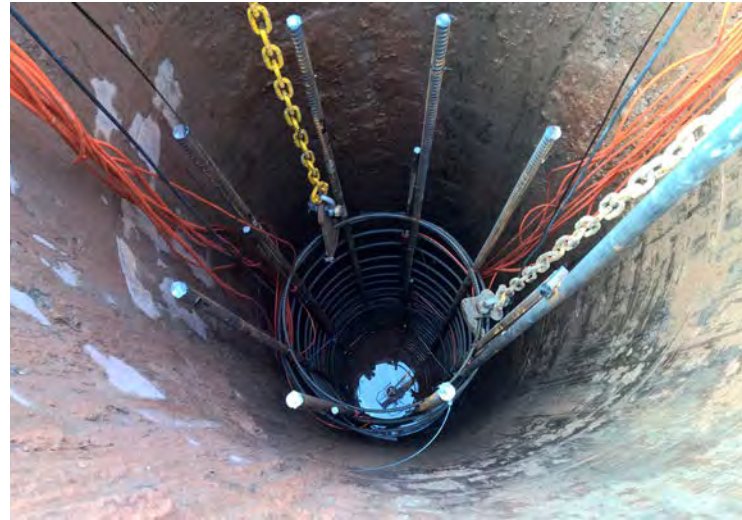
7: The piles were designed to ensure the structure met the settlement criterion, which was more than five times stricter than for a typical building
